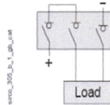
3 极 (750VDC): 两极串联为正极
